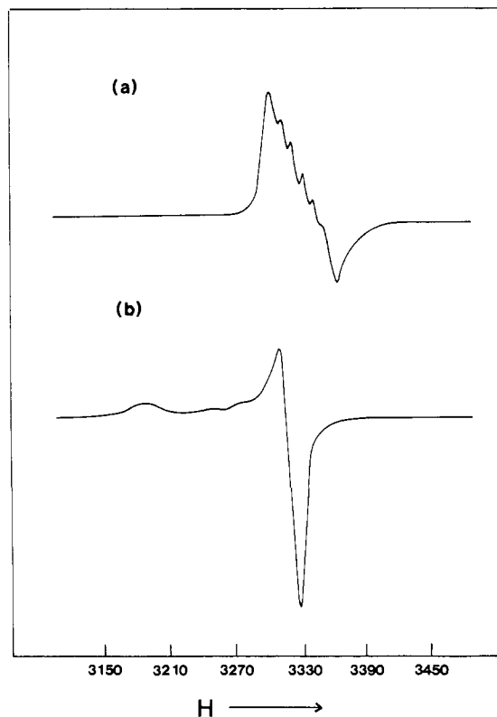
Figure 3. Frozen ESR spectra recorded after exhaustive bulk electrolysis at -1.30 V of solutions containing (a) 1.0 \times 10^{-3} M (TPP)InClO 4 and (b) 1.0 \times 10^{-3} M (TPP)In(W(CO) 3 Cp) in CH 2 Cl 2 , 0.1 M TBAP.
