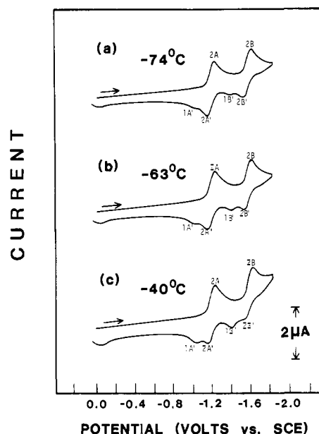
Figure 2. Temperature-resolved cyclic voltammograms of 0.9 \times 10^{-3} M (TPP)In(Mo(CO) 3 Cp) in CH 2 Cl 2 , 0.1 M TBAP. Scan rate = 100 mV/s. Temperature: (a) -74, (b) -63, and (c) -40 °C.
